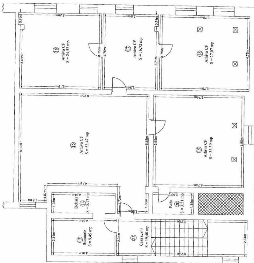
PLAN MANSARDA
